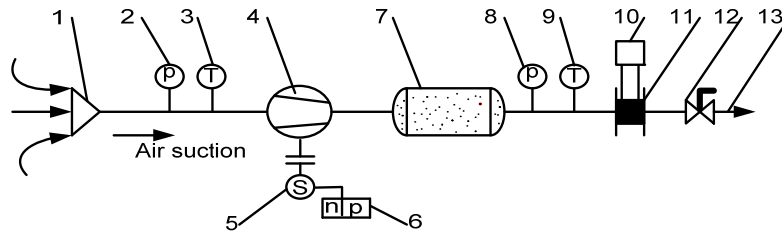
Fig.9. The experimental installation scheme for testing a rotating blower with profiled rotors 1 air filter; 2-device for measuring the pressure at the blower suction; 3- air temperature measuring device; 4-rotating blower; 5-electric motor; 6-panel with electrical appliances; 7- compressed air tank; 8-manometer with digital display; 9-thermometer with digital display; 10-differential manometer; 11- diaphragm; 12- control; 13 DN 50 air discharge valve.
