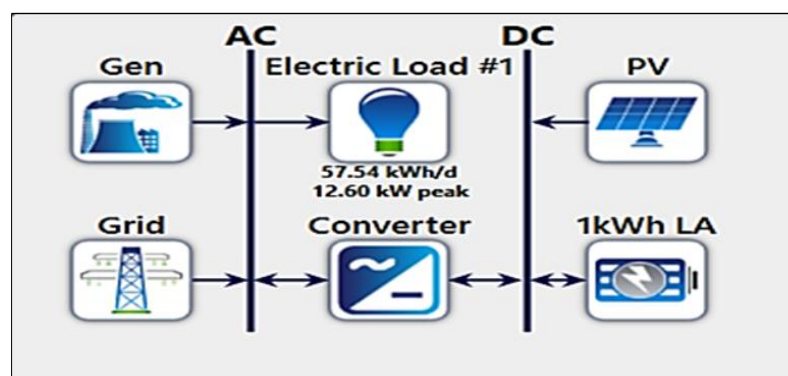
Figure 4. Schematic of the proposed hybrid power system
