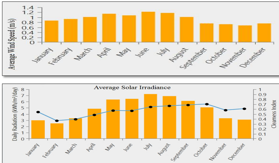
Figure 3. The annual solar irradiation and wind speed in East Karbala [12]
