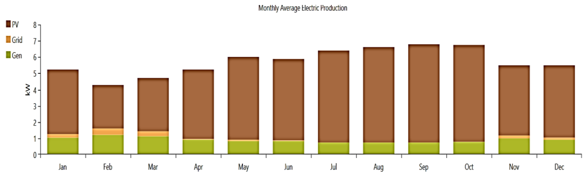
Figure 8. The penetration level of each component in the second hybrid power system
