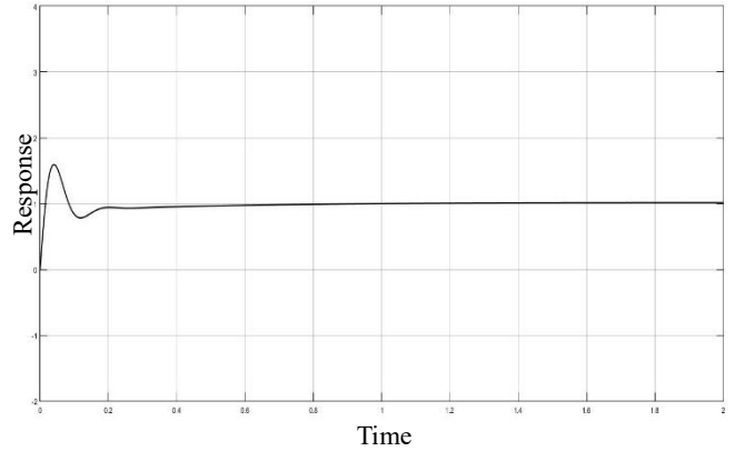
Figure 7 Closed loop system response with Fuzzy logic
