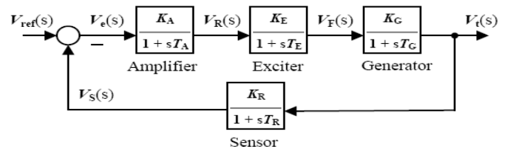
Figure 1 feedback control system with AVR
