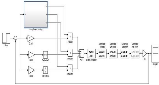
Figure 4. Feedback control system for 4 th order AVR with proposed controller
