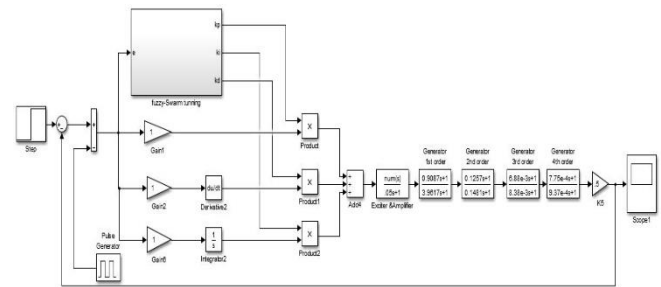
Figure 9 Closed loop system response of AVR system subjected to disturbance simulated in Matlab-Simulink
