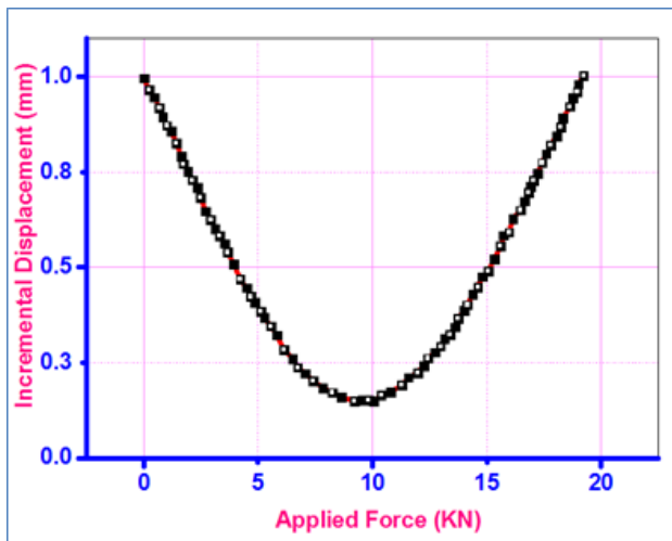
"Fig. 15". Relationship between nodal incremental displacement and force.
