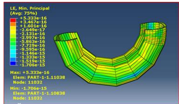
"Fig. 8". Contour of logarithmic strain
