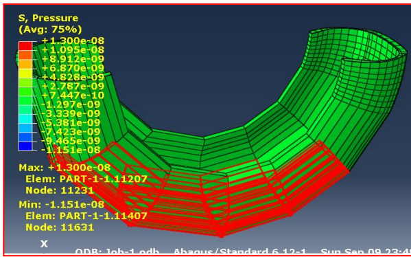
"Fig. 9". Contour of pressure distribution.
