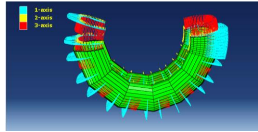
"Fig. 12". Contour plot of material orientation.
