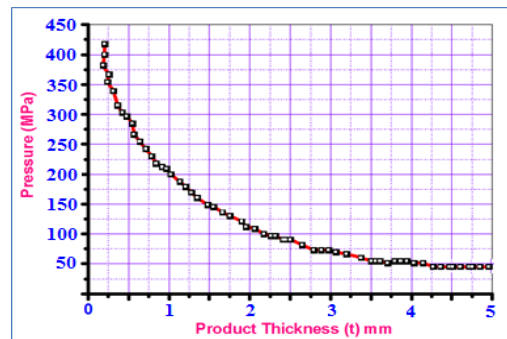
"Fig.13". Sensitivity of product thickness to the applied pressure.
