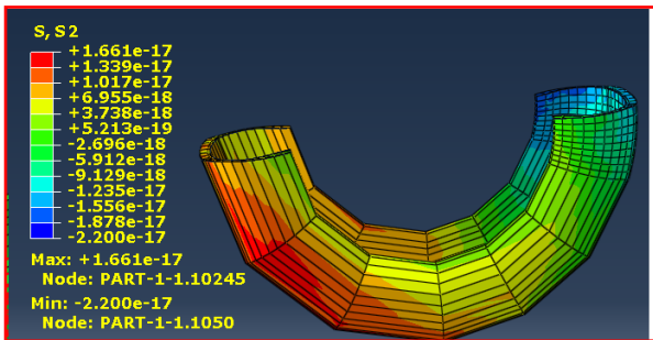
"Fig. 10". Contour of horizontal stresses.
