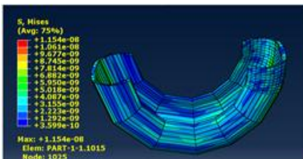
"Fig. 11". Contour plot of Von-mises stresses.
