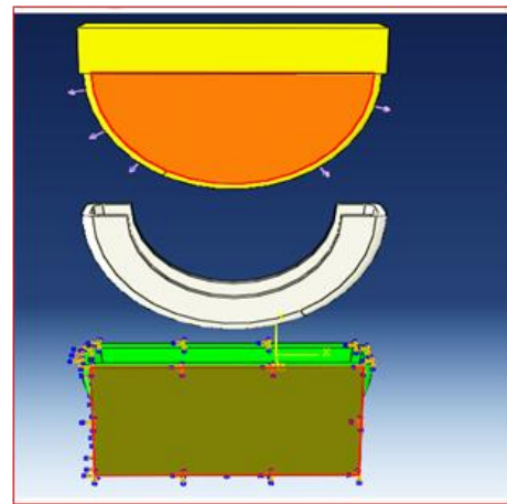
"Fig. 3". Boundary conditions on the assembly model.
