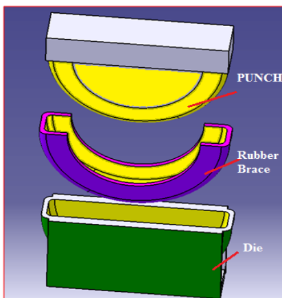
"Fig. 2". Assembly model of tools used in forming the rubber pad. Conclusions
