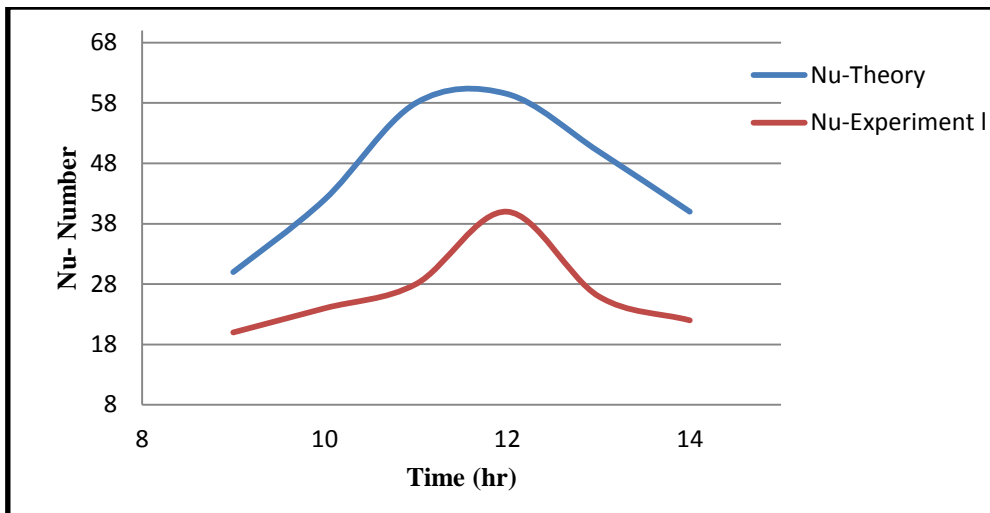
Fig.(6): Nu along the collector during Cloudy day
