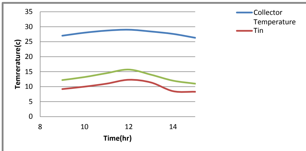
Fig.(3) : Temperatures inlet , outlet and Collector temperature during the Cloudy day
