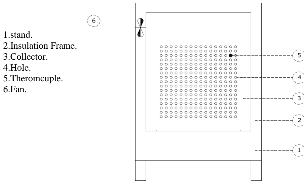
Figure (1): The test rig:
