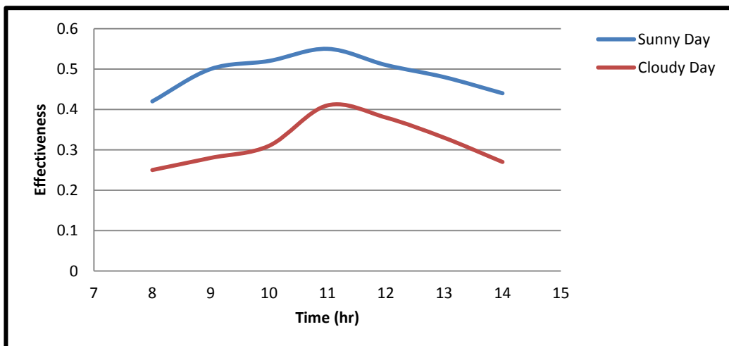
Fig.(4):Collector Effectiveness At Sunny And Cloudy Day
