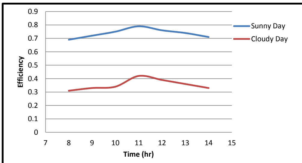
Fig.(7) :Collector Efficiency at Sunny and Cloudy Day
