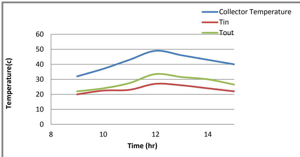
Fig.(2) : Temperatures inlet , outlet and Collector temperature during the Sunny day
