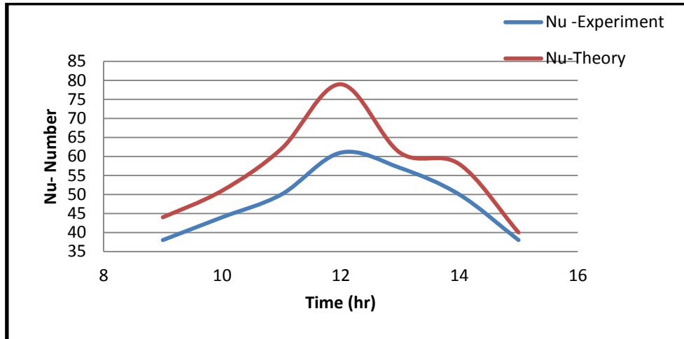
Fig.(5): Nu along the collector during Sunny day
